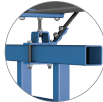
Standard assembly (upper/lower hanger bracket)
