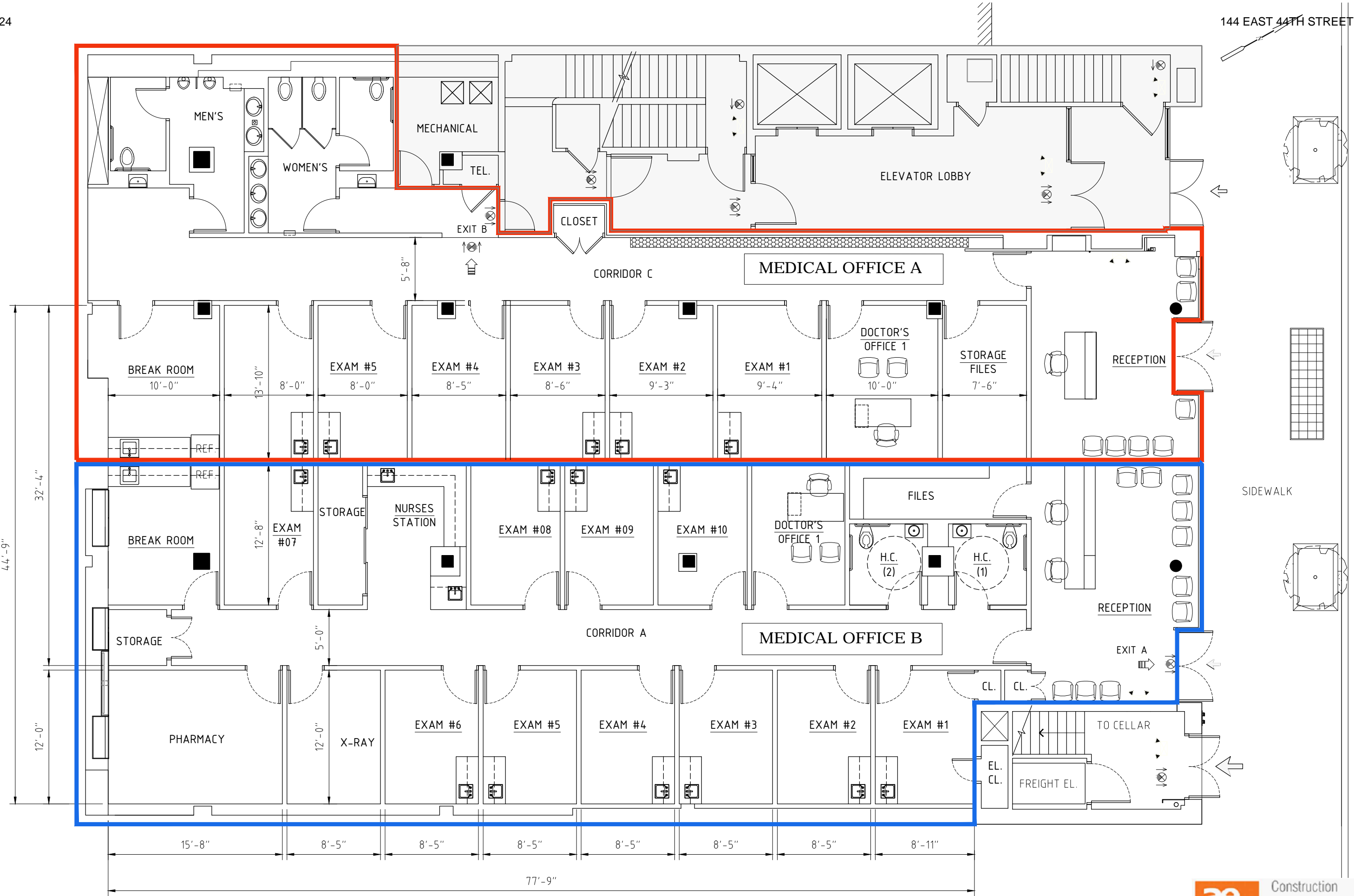
FIRST FLOOR PLAN - C
