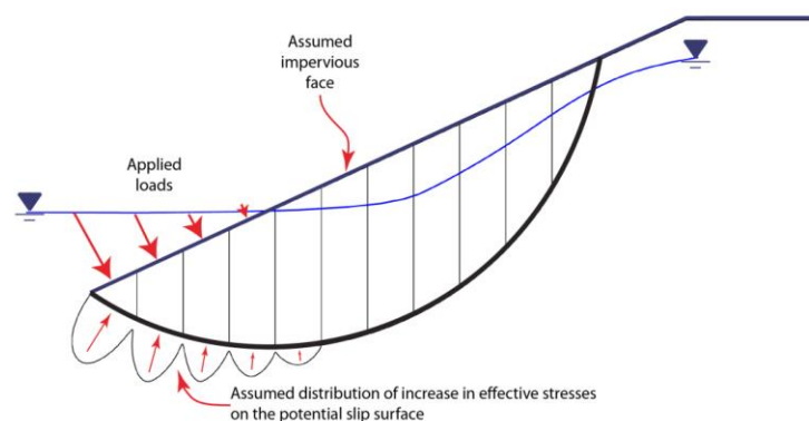
Figure 4 – Application of Pond Pressures
