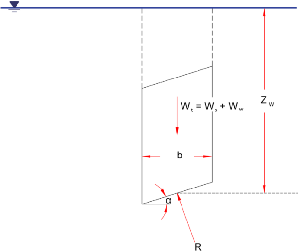
Figure 1 – Hydrostatic condition
