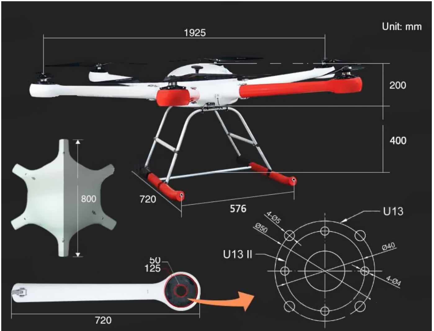
Airframe dimensions
