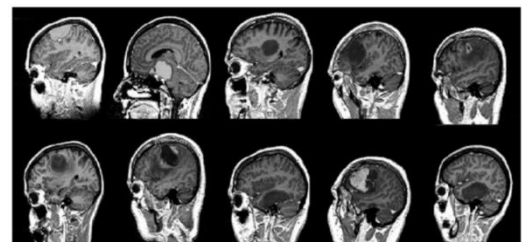
Figure 1: DATASET
