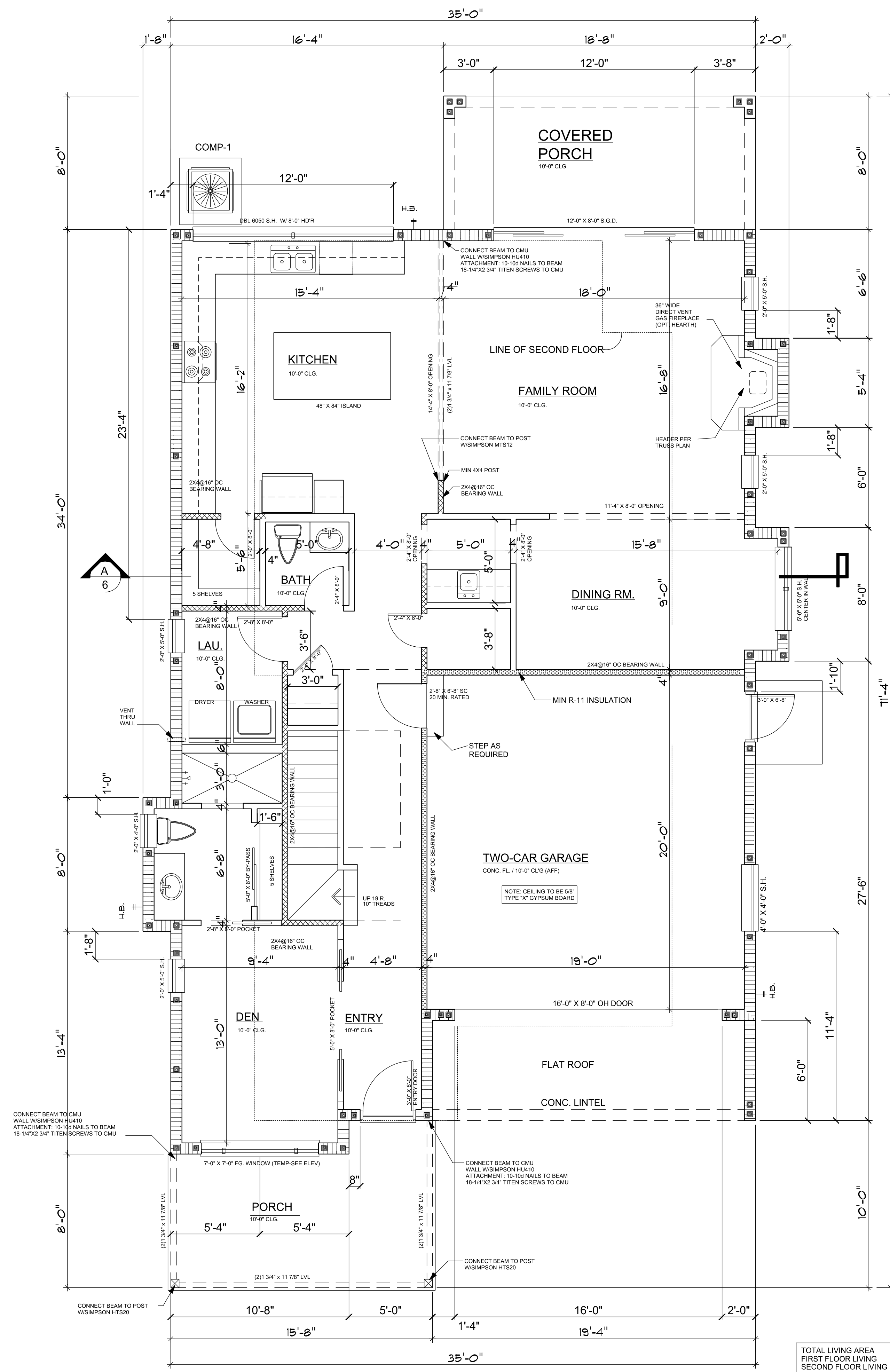
FIRST FLOOR - FLOOR PLAN 1/4" = 1'-0"
