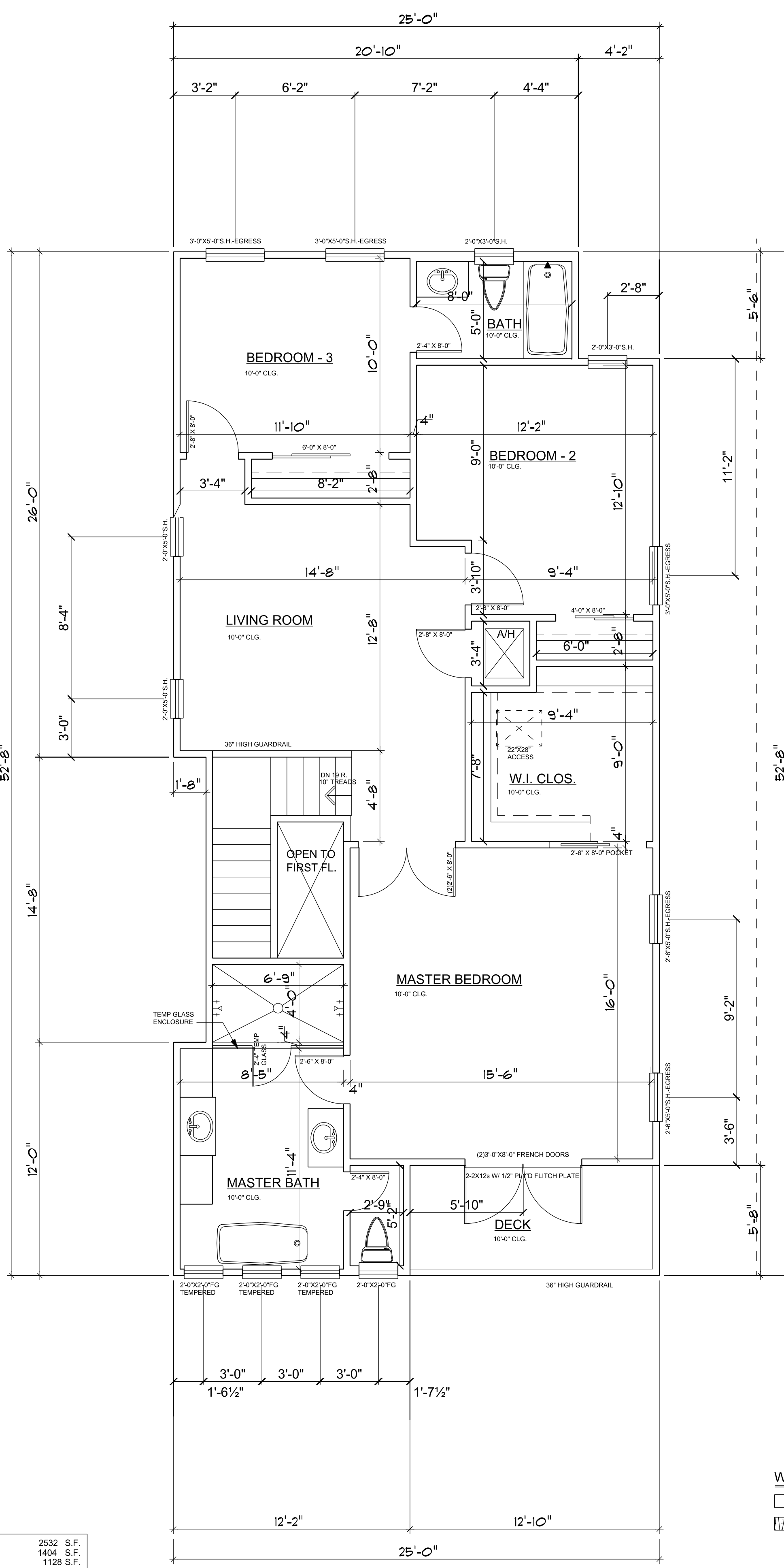
SECOND FLOOR - FLOOR PLAN 1/4" = 1'-0"
