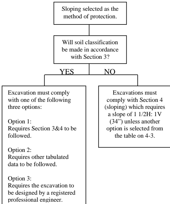
Figure 2. Sloping Options
