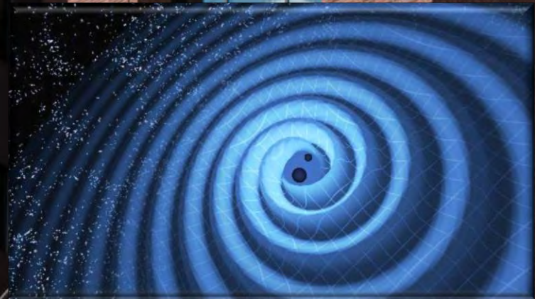
Gravitational Waves
