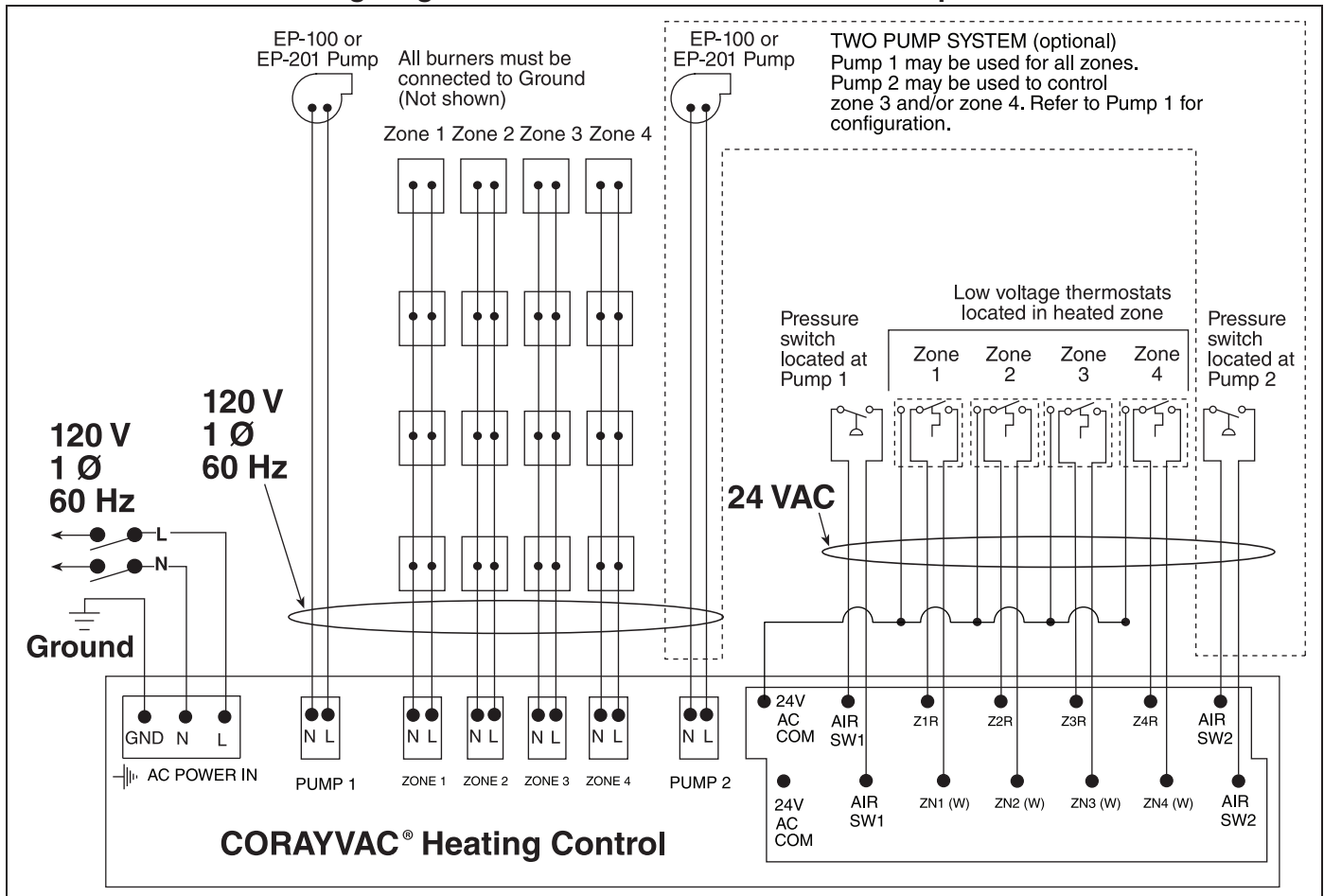
FIGURE 41: External Wiring Diagram EP-100 and EP-201 120 V 1 Ø Pump
