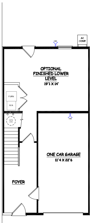
LOWER LEVEL PLAN
