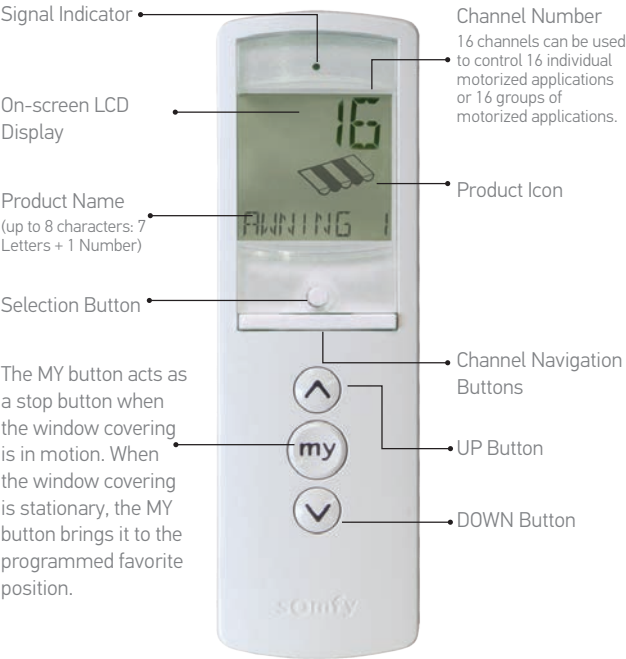
Telis 16 RTS Pure 16 Channel Hand-held Remote 1811081
