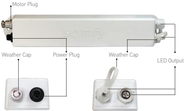
LED 12V Light Control Kit Warm White 1811491 LED 12V Light Control Kit Warm White 1811506
