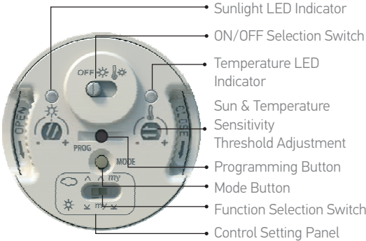
Front view with cover removed
