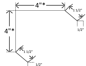
Corner
