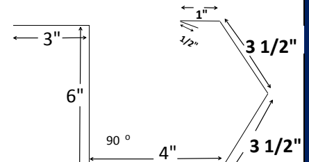
Standard Gutter
