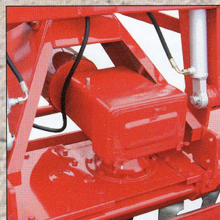
Selectatilt gearbox.
