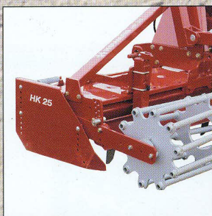
Depth adjustment and side deflector.
