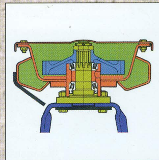
Frame and rotor unit.
