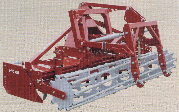
HK 25 with crumble roller and hydraulic Hitch (optional).
