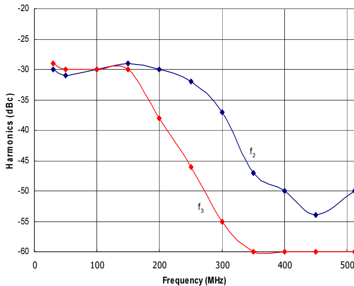
Figure 3: RFMS30-512-20 Typical f_2 and f_3 @ P_{out} = 20W .
