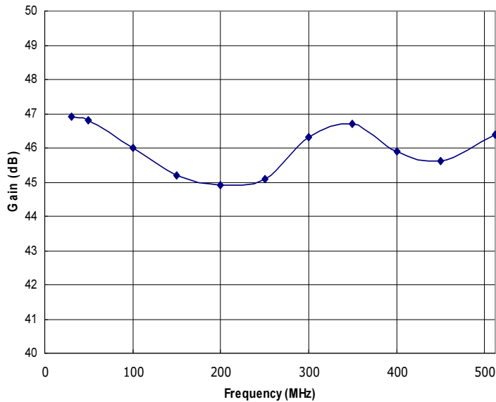
Figure 1: RFMS30-512-20 Typical Gain @ P_{out} = 20W .
