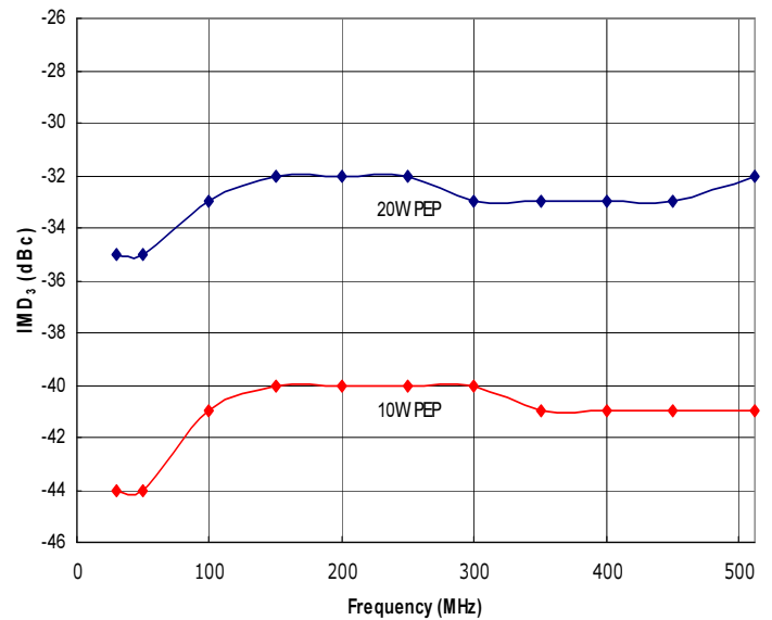
Figure 2: RFMS30-512-20 Typical IMD_3 , \Delta f=10kHz , @ P_{out} = 20W and 10W PEP.
