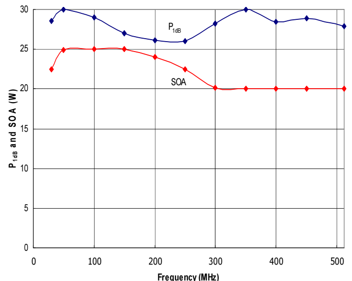
Figure 4: RFMS30-512-20 Typical P_{1dB} and Safe Operating Area (SOA). The amplifier is capable of delivering more power than it is safe to generate. Do not exceed the SOA without first contacting RFMPT to discuss your application.
