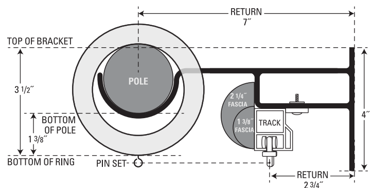
2 1/4" Pole & Traverse Rod Combination Bracket - 20-297 Bracket must be specified with order.
