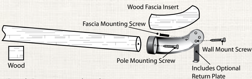
13-463-17 Bronze Wood Fascia Finish with Bronze Metal Return
