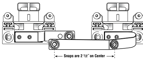
Center of Snap Locations
