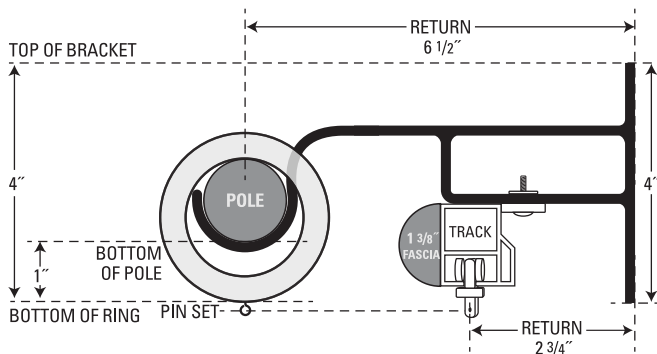
1 3/8" Pole & Traverse Rod Combination Bracket - 10-296 Bracket must be specified with order.
