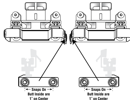
Premium Ripplefold® Butt Master
