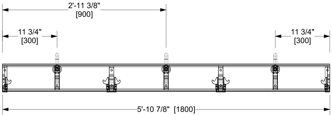
1 Front View 1:10
