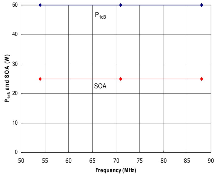
Figure 4: RFP54-88-25 Typical P 1dB and Safe Operating Area (SOA). The amplifier is capable of delivering much more power than it is safe to generate. Do not exceed the SOA shown above.
