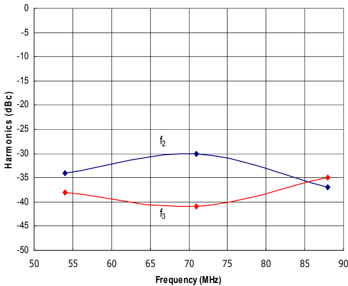
Figure 3: RFP54-88-25 Typical f 2 and f 3 @ P out = 25W.
