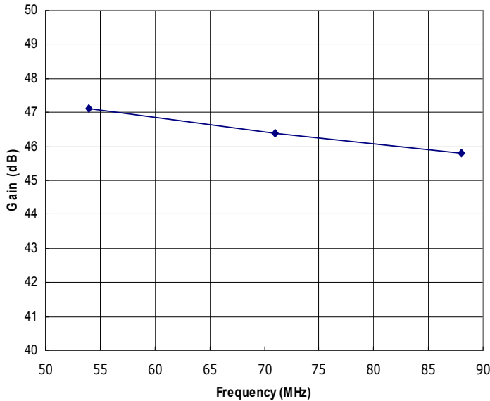
Figure 1: RFP54-88-25 Typical Gain @ P out = 25W.
