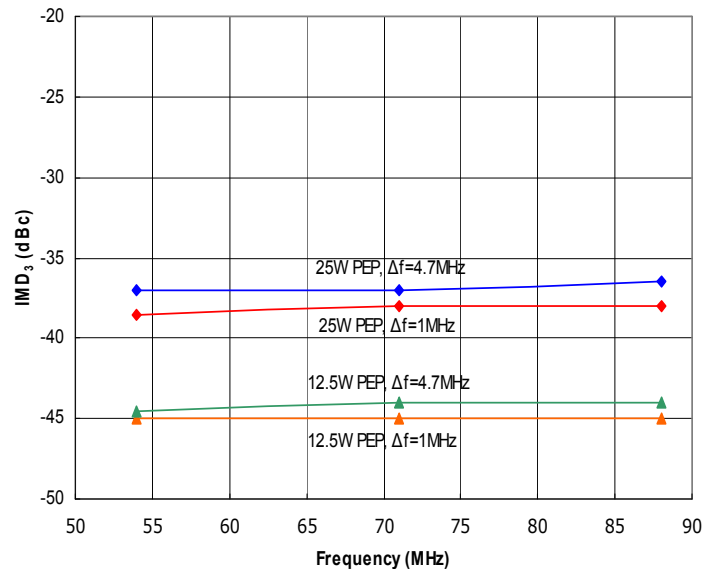
Figure 2: RFP54-88-25 Typical IMD 3 @ 25W and 12.5W PEP, Δf=1MHz and Δf=4.7MHz.
