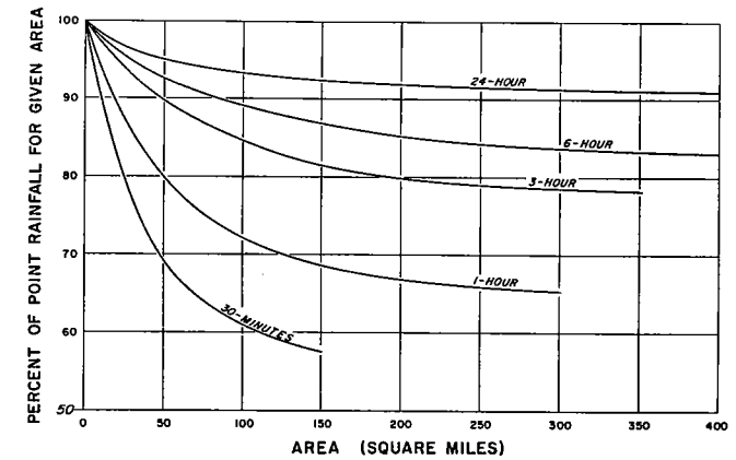
FIGURE 15.—Area-depth curves.
