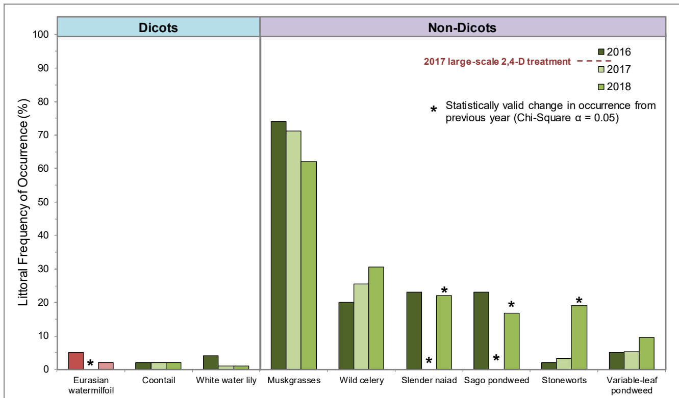
Figure 5.5-2. Littoral frequency of occurrence of aquatic plant species from 2016-2018 in Dake Lake. Data from Onterra 2016-2018 Point-Intercept Surveys. Whole-lake 2,4-D herbicide treatment occurred in spring 2017.
