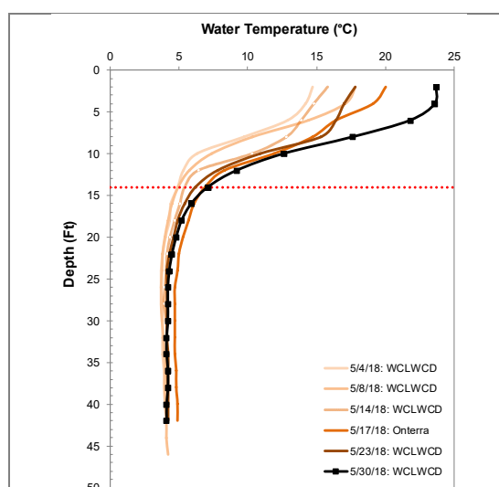
Figure 3.2-2 Pre-Treatment Temperature Profiles Collected on Beasley Lake. Red dashed line indicates dosing depth.
