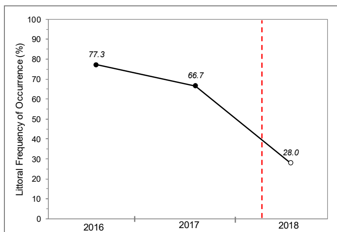
Figure 5.3-1. Littoral Frequency of Occurrence of HWM in Bass and Beasley Lakes from 2016-2018. Data from Onterra 2016-2018 Point-Intercept Surveys. Red dashed line indicates whole-lake treatment. Open circle indicates statistically valid difference from previous survey.
