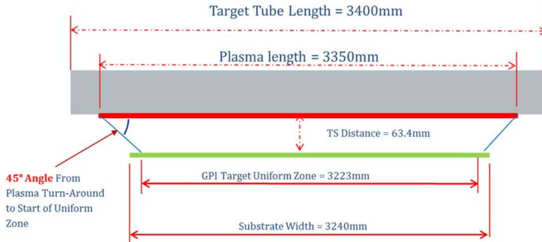
Figure 7. Expanded Uniformity Zone of Rotary Target with New Magnet Bar Design
