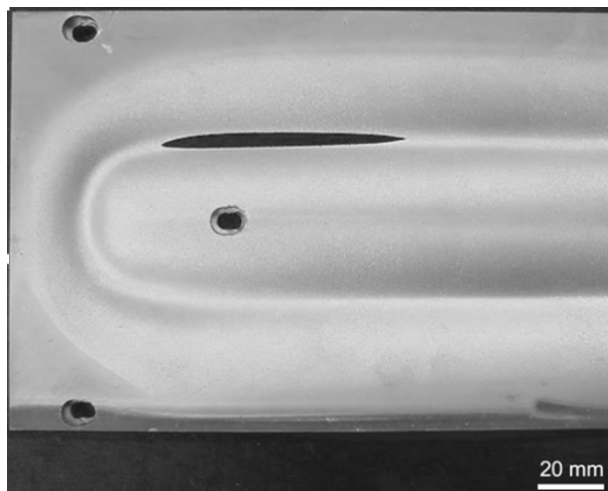
Figure 2. Typical Planar Magnetron Target Erosion at Turn-around due to "Cross-corner" Effect
