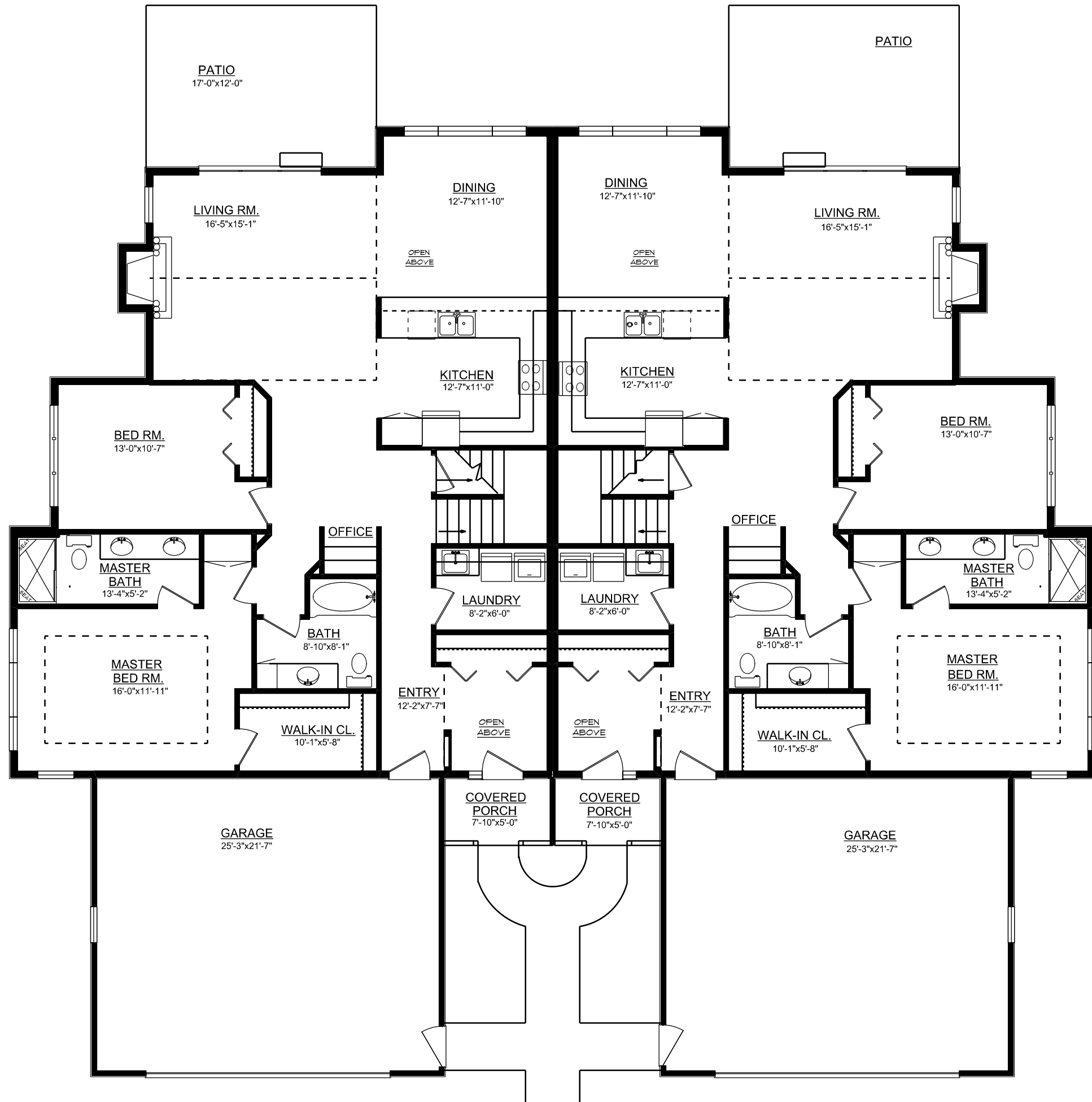
FIRST FLOOR PLAN 1661 SQ.FT. @ 1ST.FLOOR EACH UNIT
