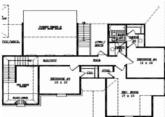
SECOND LEVEL FLOOR PLAN
