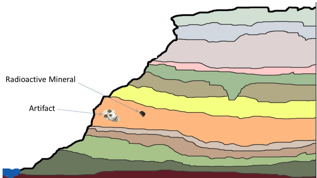
Figure 13: Stratigraphy
