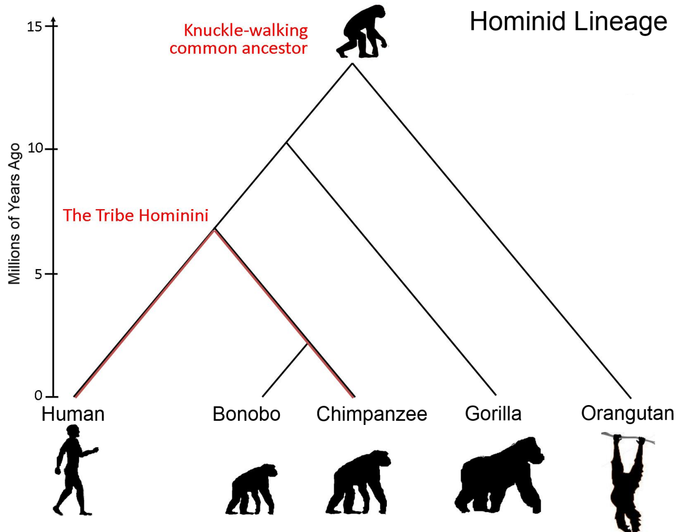
Figure 1: Hominid cladogram
