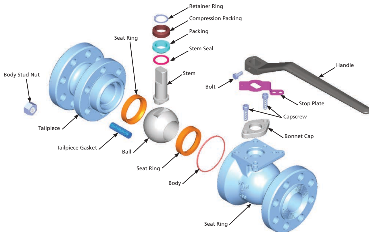
Flanged Ends 310F
