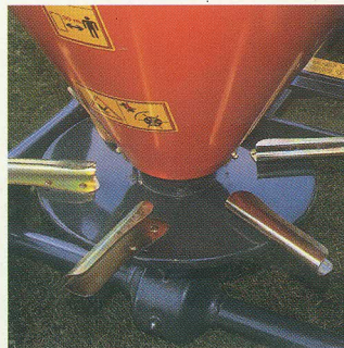
Spreading disc with adjustable vanes.
