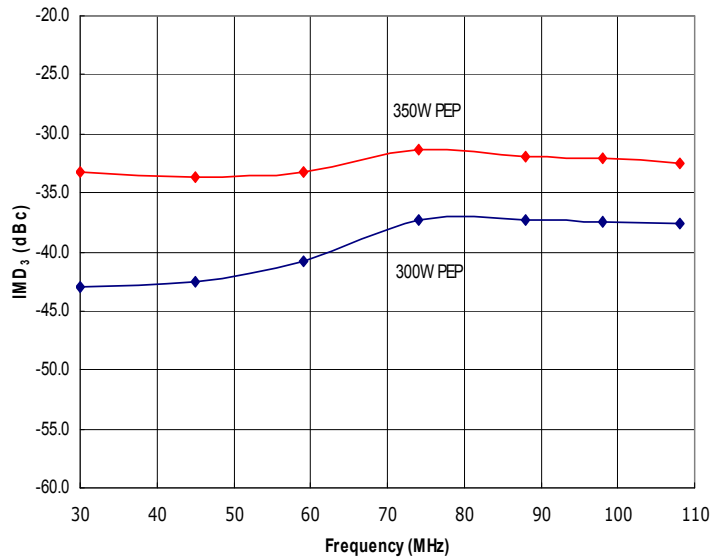
Figure 2: RFM30-108-350-HSD Typical IMD 3 @ 350W and 300W PEP, Δf = 100kHz.
