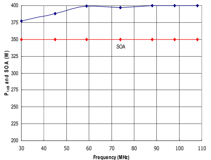
Figure 4: RFM30-108-350-HSD Typical P 1dB and Safe Operating Area (SOA). The amplifier is capable of delivering more power than it is safe to generate. Do not exceed the SOA shown above without first contacting RFMPT to discuss your application.
