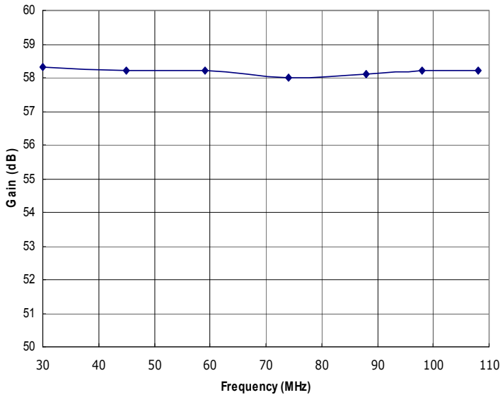
Figure 1: RFM30-108-350-HSD Typical Gain @ P out = 350W.
