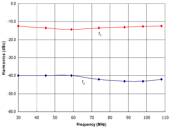
Figure 3: RFM30-108-350-HSD Typical f 2 and f 3 @ P out = 350W.
