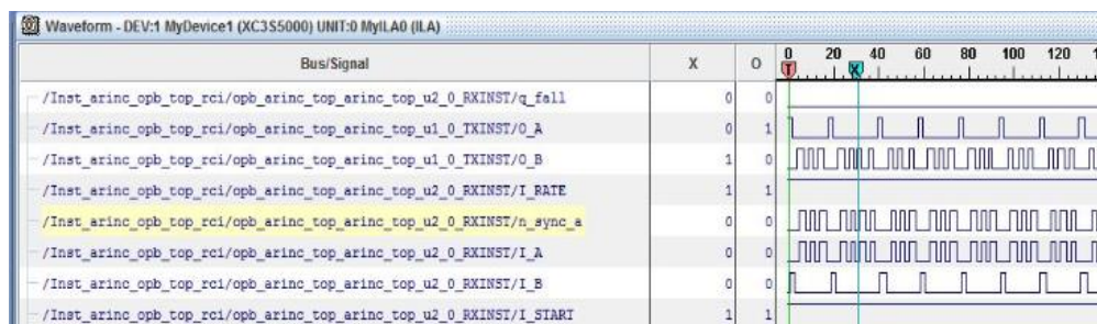
Fig. 6.7: chip scope resultant wave
