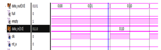
Fig. 6.2: FIFO logic
