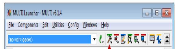
Fig. 5.1: Launcher screen
