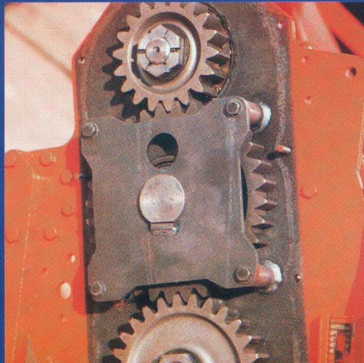
Strong side drive gears. The center gear is fitted with double plate. Totally reliable.
