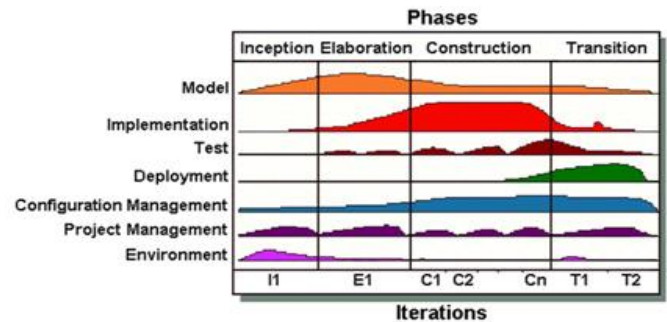
Figure 1: Agile Unified Process Model Phases
