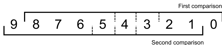
Figure 6: Testing for break in mean
