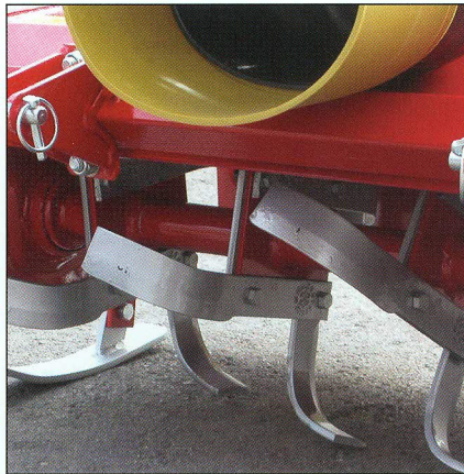
The rotor with blades 9941/42 is very effective.
