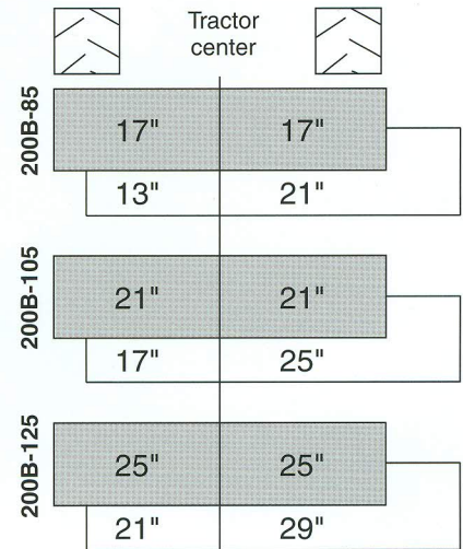
Rotavator 200-105. Specially designed for compact tractors.
