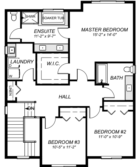
UPPER FLOOR PLAN 1161 sq ft
