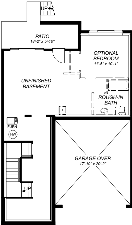
LOWER FLOOR PLAN 896 sq ft
