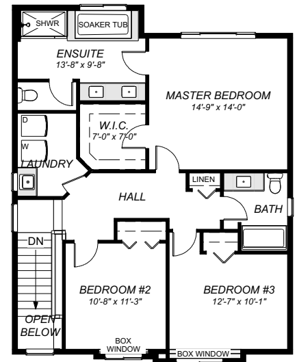
UPPER FLOOR PLAN 1060 sq ft
