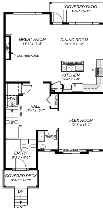
MAIN FLOOR PLAN 1215 sq ft
