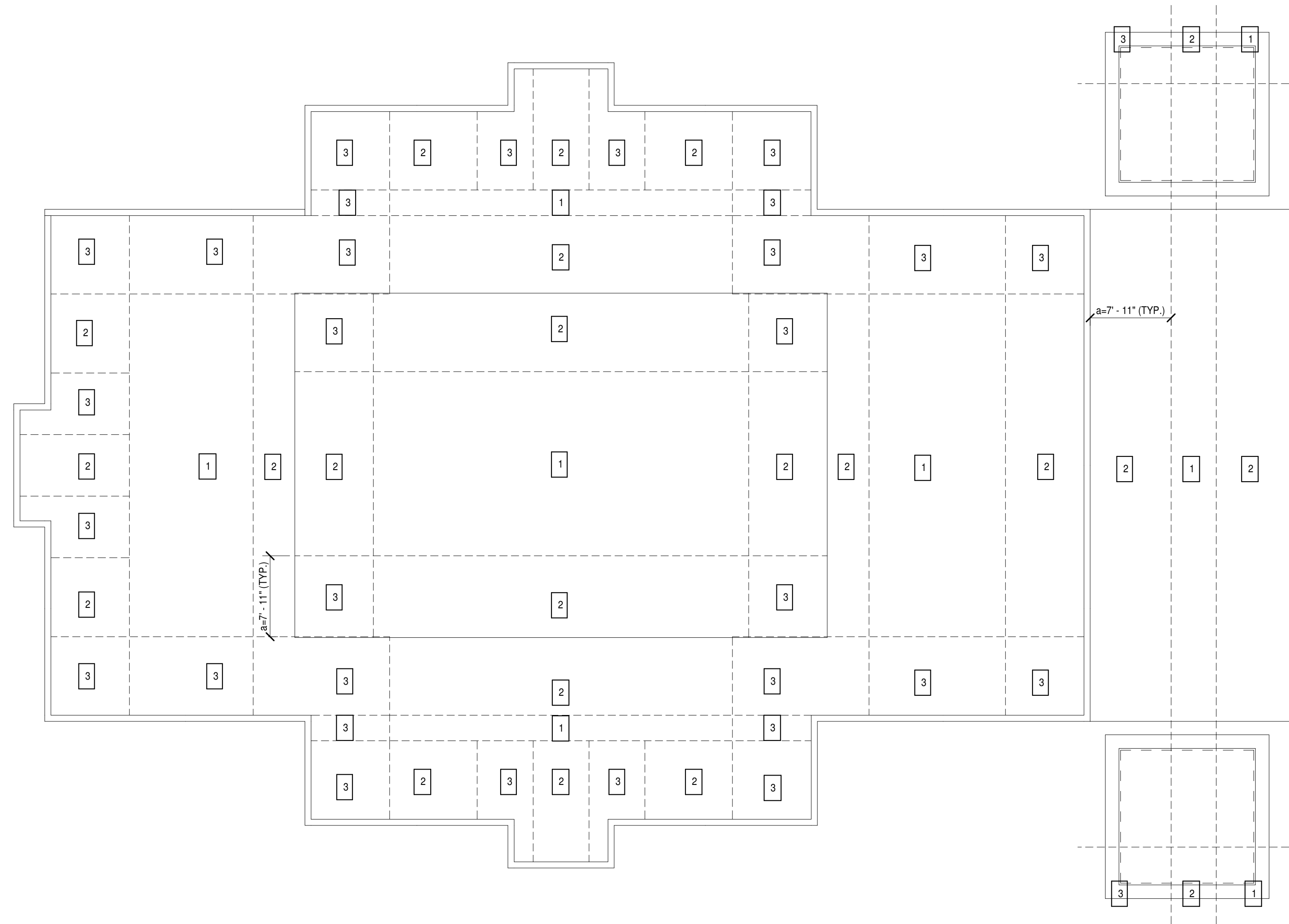
1 WIND PRESSURE DIAGRAM (GROSS VALUES) S3.0A 1/8" = 1'-0"
