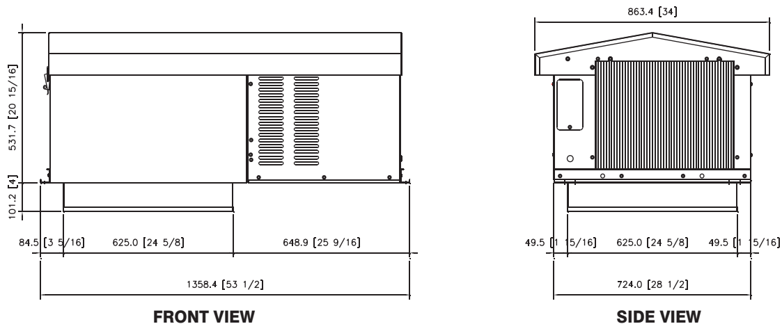
Figure B. OUTDOOR UNIT – Medium Cabinet (Opening Size : 25 inch x 25 inch)
