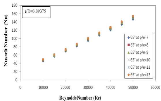
Fig.4.3. Variation of Nusselt number with Reynolds number (10000 - 50000) for different pitch roughness ( p/e = 7, 8, 9, 10, 11, 12 ) at 65°.
