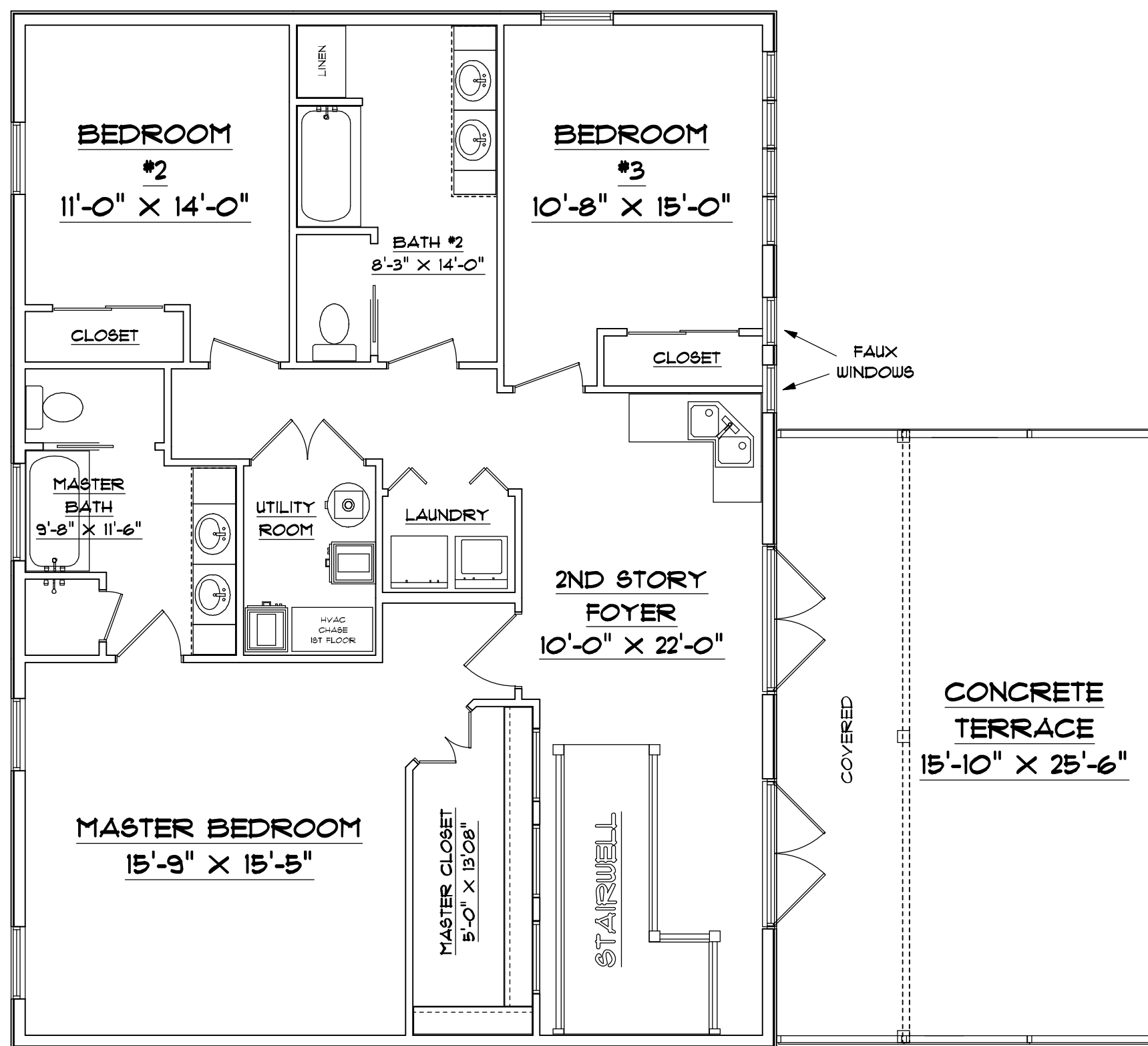
2ND STORY
