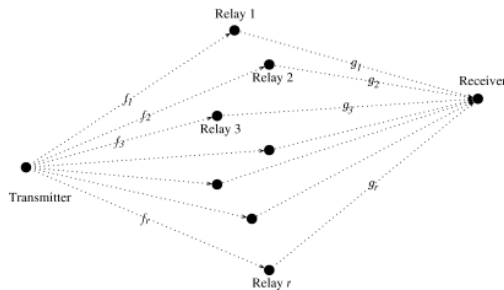
Fig.1: MIMO-Relay Path Process
