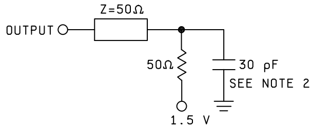
CIRCUIT A
