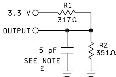
CIRCUIT B
