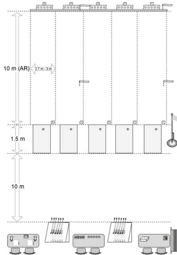
Figure 10B-2 Recreational Summer Biathlon Air Rifle Range Layout
