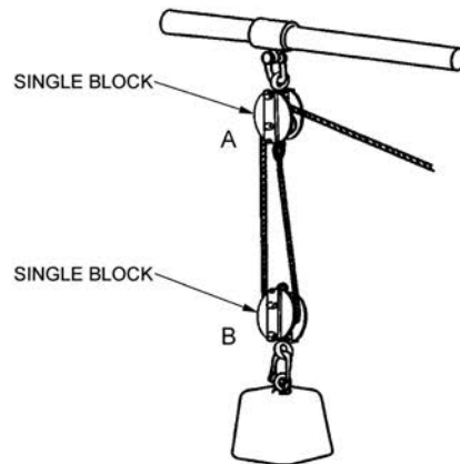
Figure 11-5-2 Double Whip
