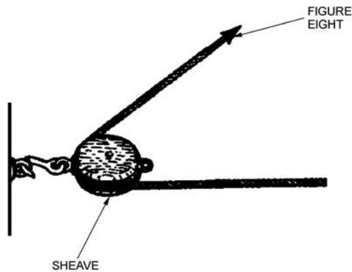
Figure 11-3-4 Reeving a Block
