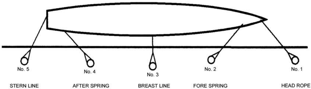
Figure 12-7-1 Berthing Lines
