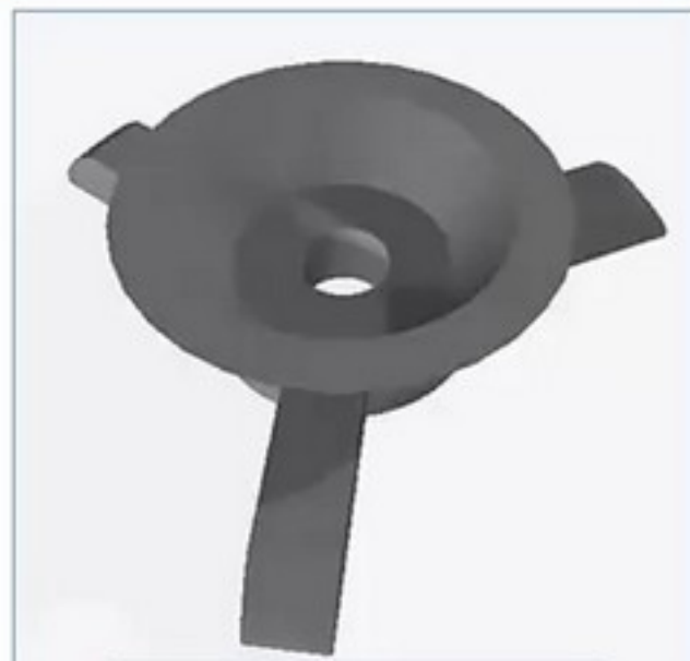
Exhaust Valve Guide and Gas Deflector
