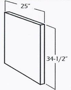
Base End Panel (5/8" thickness) BEP15mm*24
