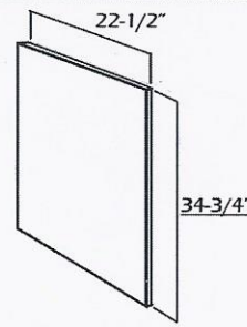
Base End Panel (1/4" thickness) BEP5mm*22.5
