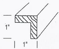
Corner Moulding OCM8
