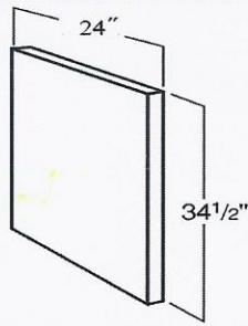
Dishwasher Panel (3/4" thickness) DWP
