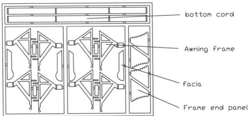
280 mm Awning Frame
