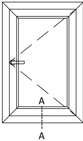
OUTSWING DOOR
