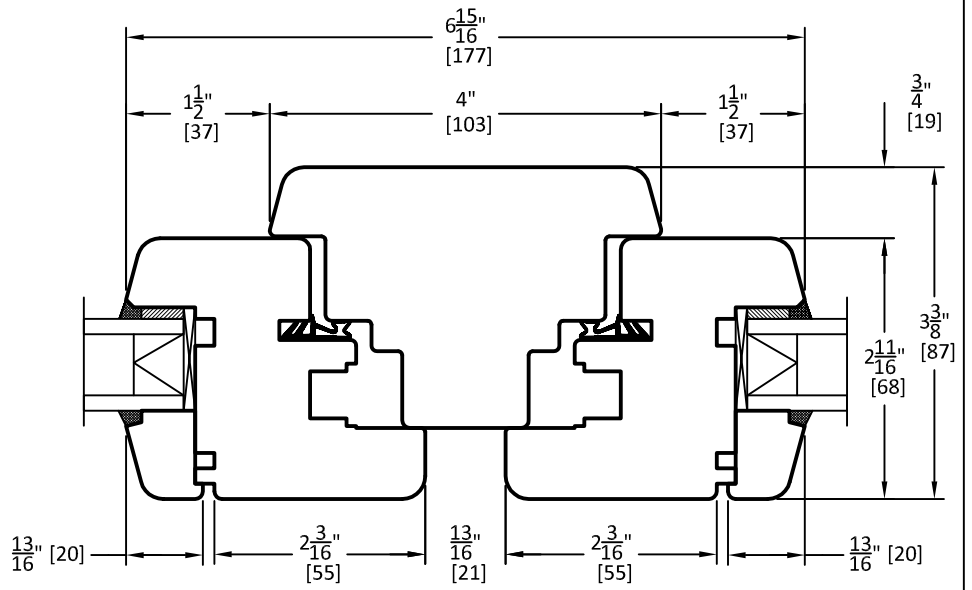
① 1" GLAZING
