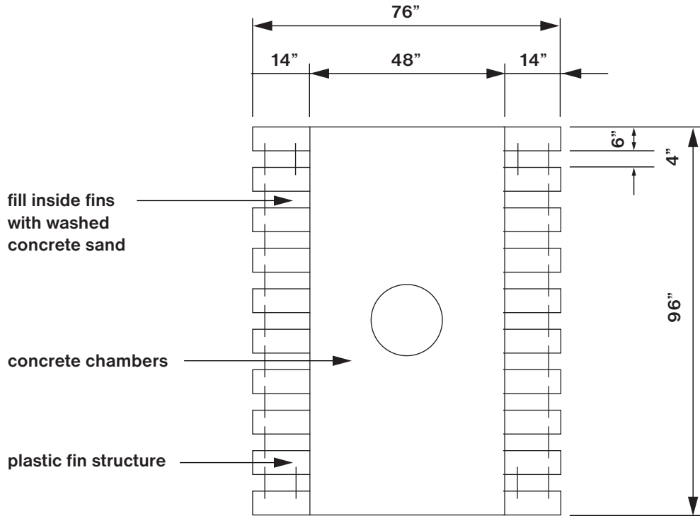
PLAN VIEW
