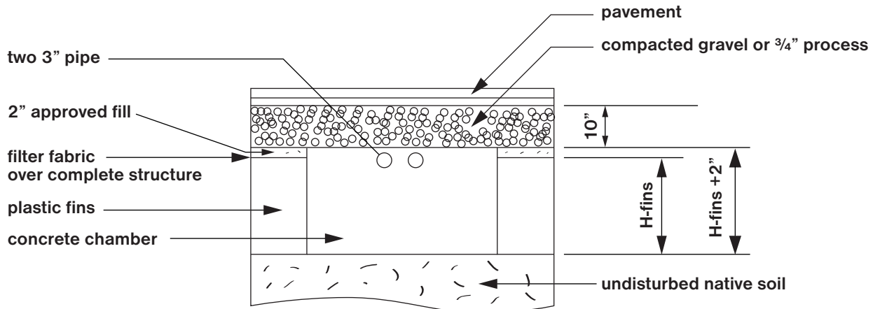
END VIEW
