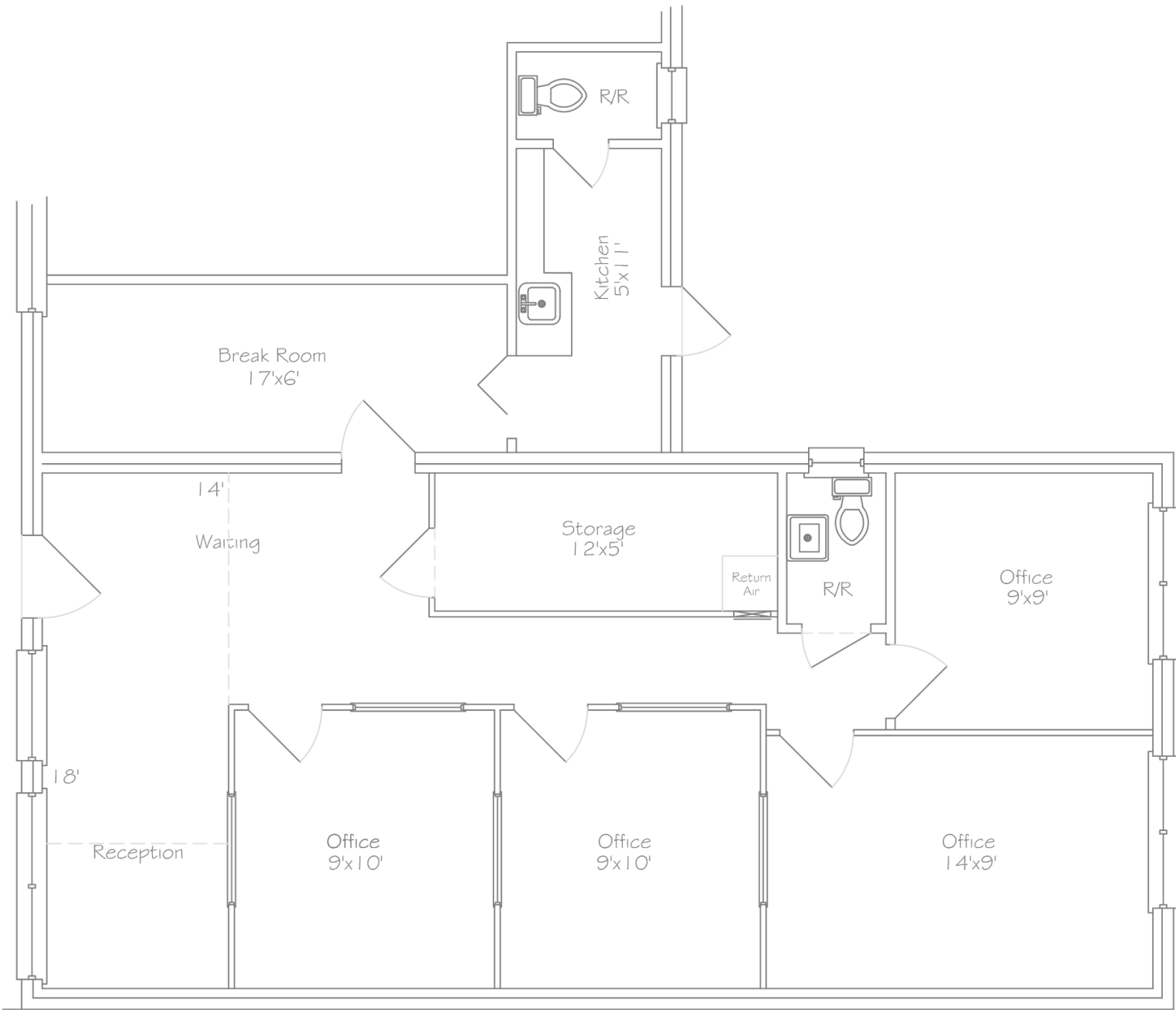
FLOOR PLAN 1,000 sq. ft.
