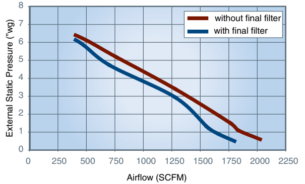
WSO 25-3 (10 HP)
