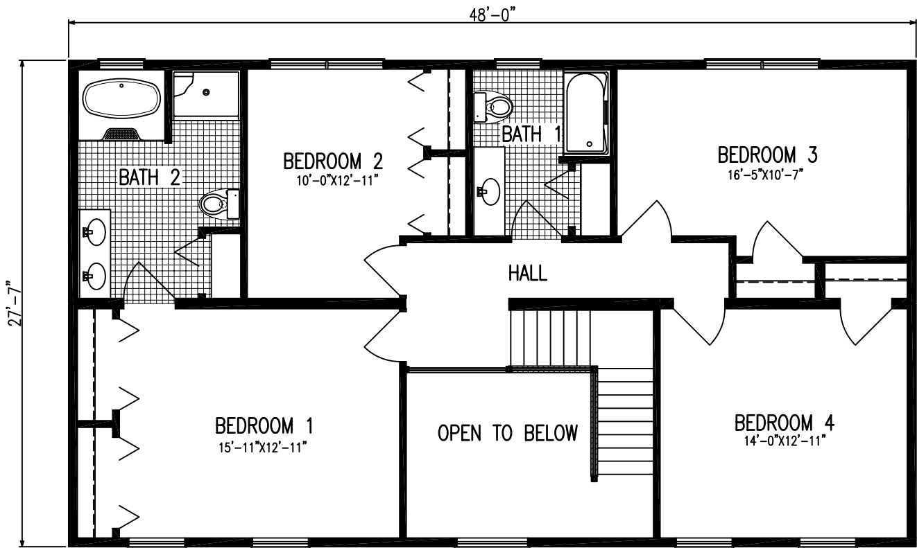
2ND FLOOR- 1344 SQ FT
