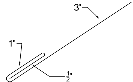
STANDING SEAM RAKE EDGE J-CHANNEL _____ LINEAR FEET (120' PCS)
