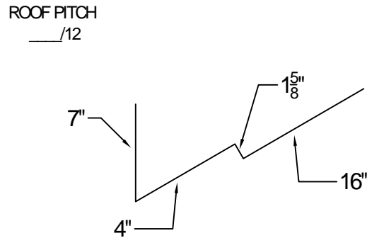
STANDING SEAM SKYLIGHT BACK _____ LINEAR FEET (120' PCS)
