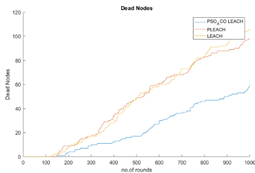
Fig.2: Number of Dead nodes in PSO_ACO Leach, PLEACH Leach and Leach
